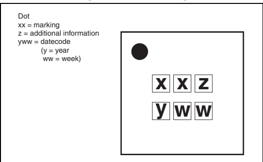
Figure 19. Marking
