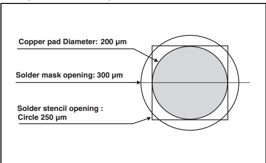
Figure 18. Footprint recommendations
