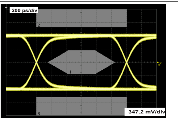
Figure 5. Eye diagram, board with USBULC6-2F7 (according to USB 2.0 high speed specification)
