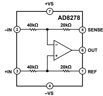
Figure 1. AD8278
