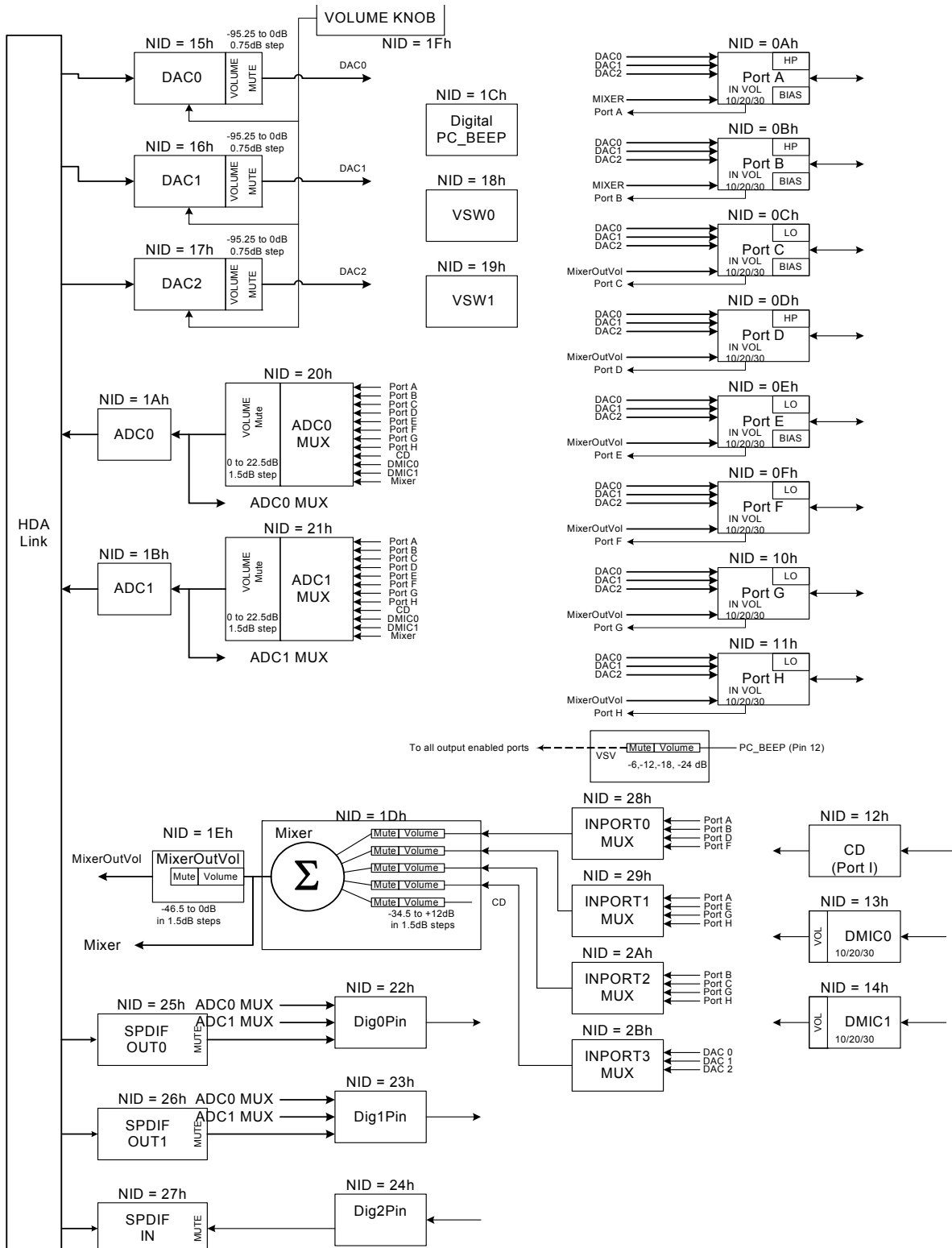
Figure 12. Widget Diagram
