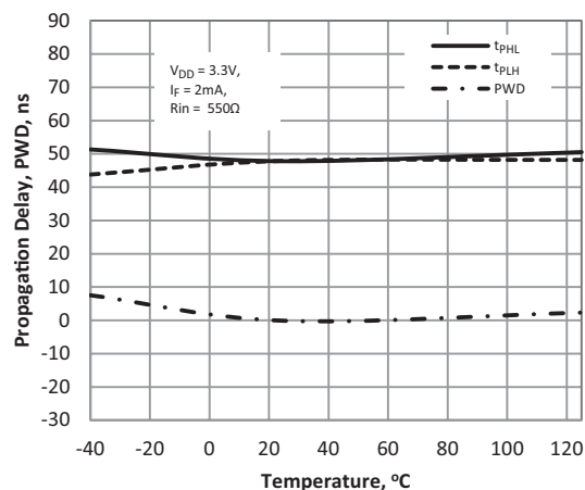
Figure 10: Typical Switching Timing (Propagation Delay, PWD) vs Temperature at 2-mA LED Driving Current, 3.3V Supply
