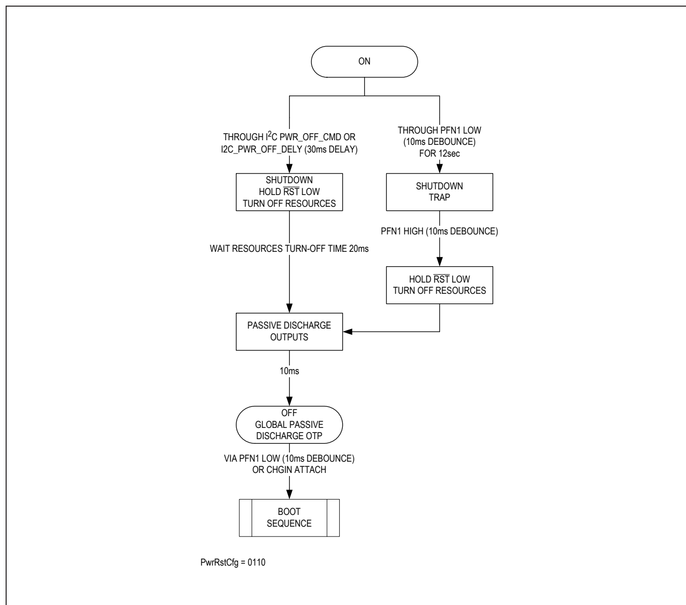
Figure 1d. PwrRstCfg = 0110
