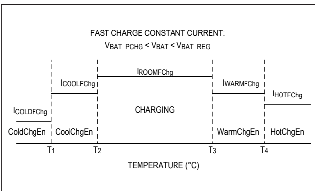
Figure 4a. Sample JEITA Pre Charge Profile
