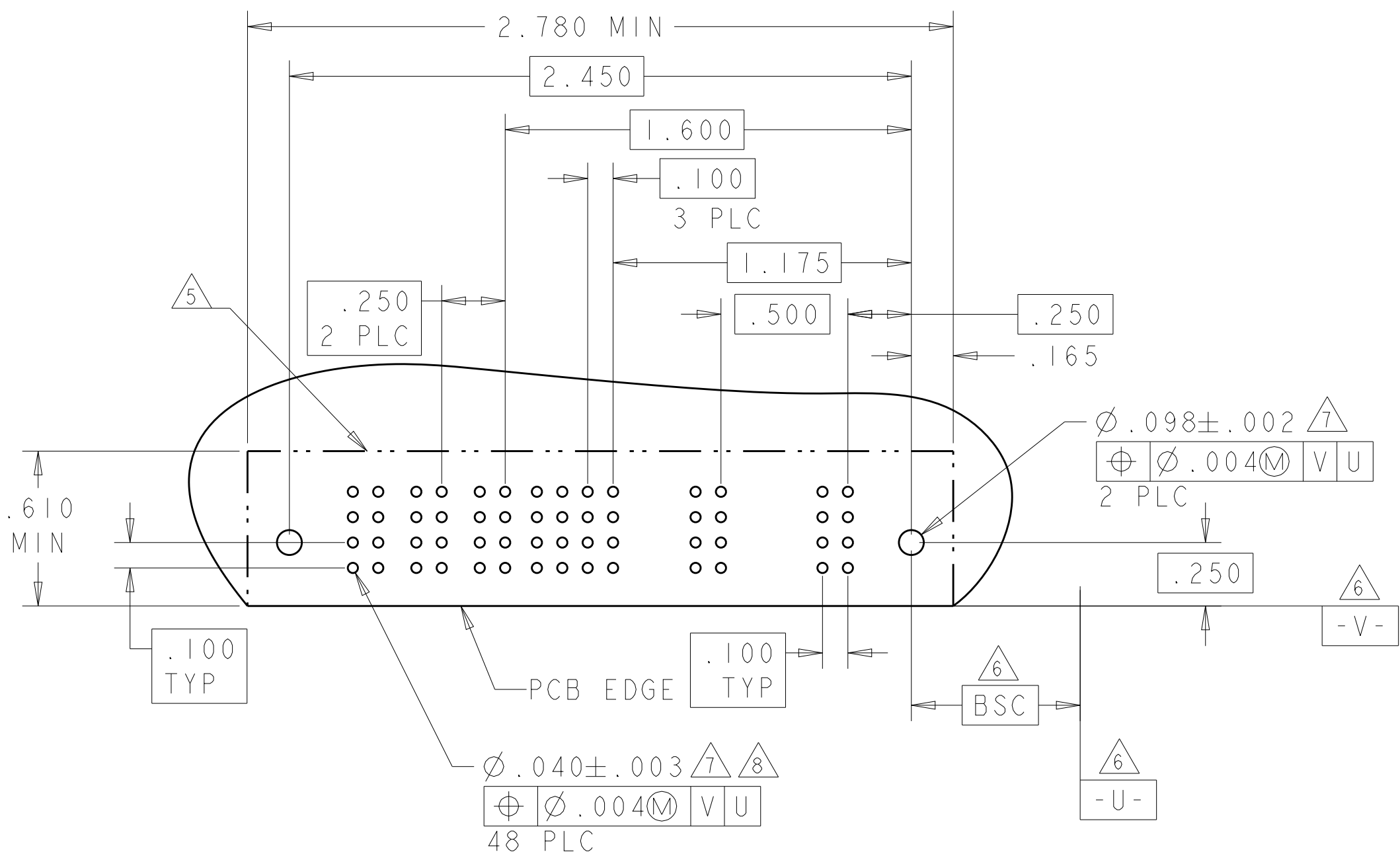
2-6450170-7 & 2-6450170-9 PCB LAYOUT
