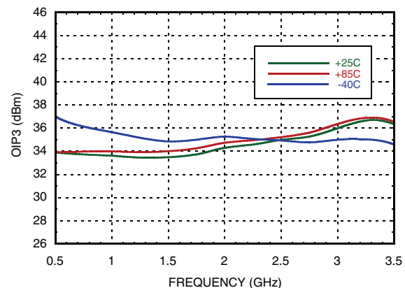
Output IP3 vs. Temperature [1]
