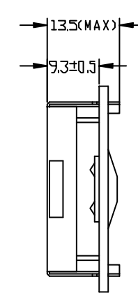
LED BKL
