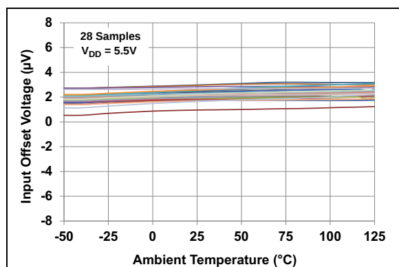
FIGURE 2: Input Offset Voltage vs. Temperature with V_{\text{DD}} = 5.5\text{V} .
