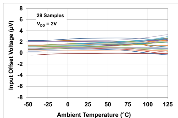
FIGURE 1: Input Offset Voltage vs. Temperature with V_{\text{DD}} = 2\text{V} .
