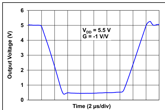
FIGURE 2-48: Inverting Large Signal Step Response.
