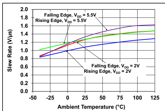
FIGURE 2-49: Slew Rate vs. Ambient Temperature.
