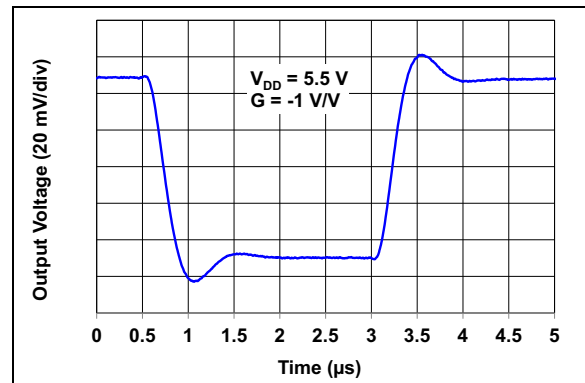
FIGURE 2-47: Inverting Small Signal Step Response.
