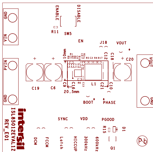
FIGURE 6. SILKSCREEN LAYER
