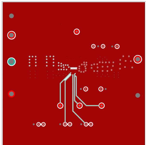
FIGURE 9. LAYER 3
