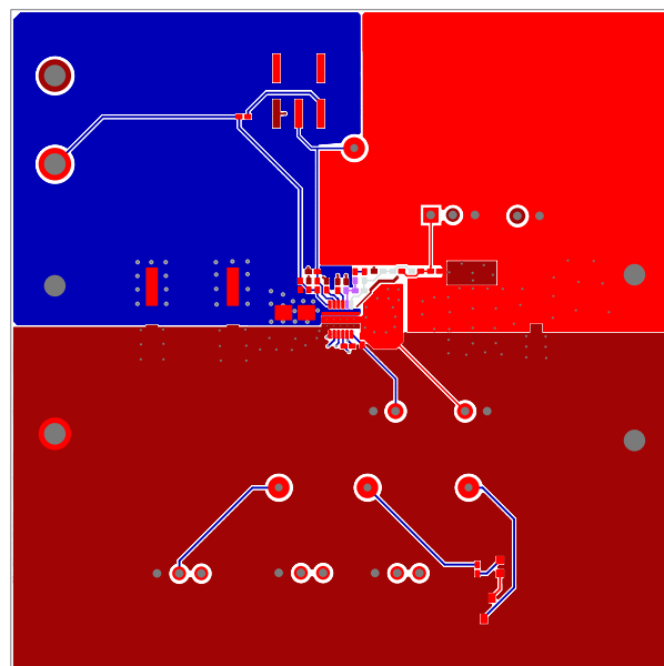
FIGURE 7. TOP LAYER
