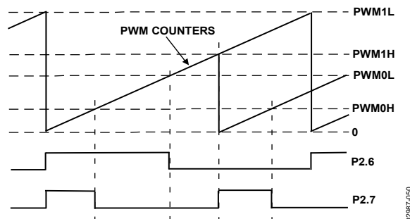
Figure 61. PWM Mode 5
