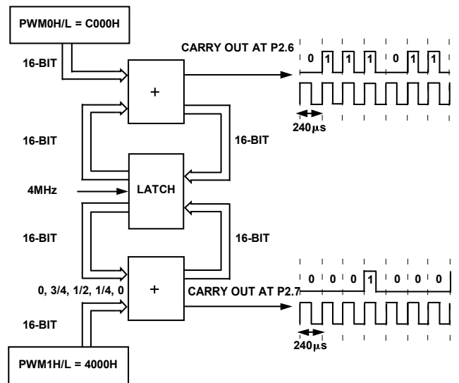
Figure 62. PWM Mode 6
