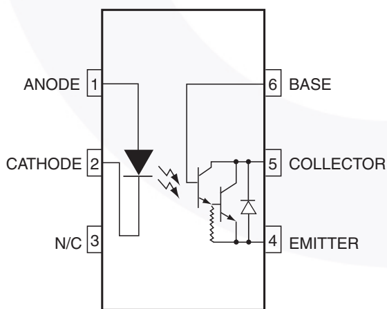
Figure 1. Schematic
