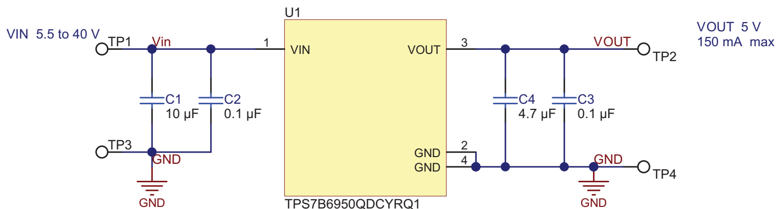
Figure 4. TPS7B6950EVM Schematic
