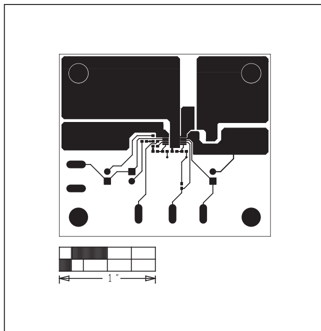
Figure 3. MAX17552 5V EV Kit (μMAX) PCB Layout—Component Side
