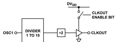
Figure 33. CLKOUT Stage
