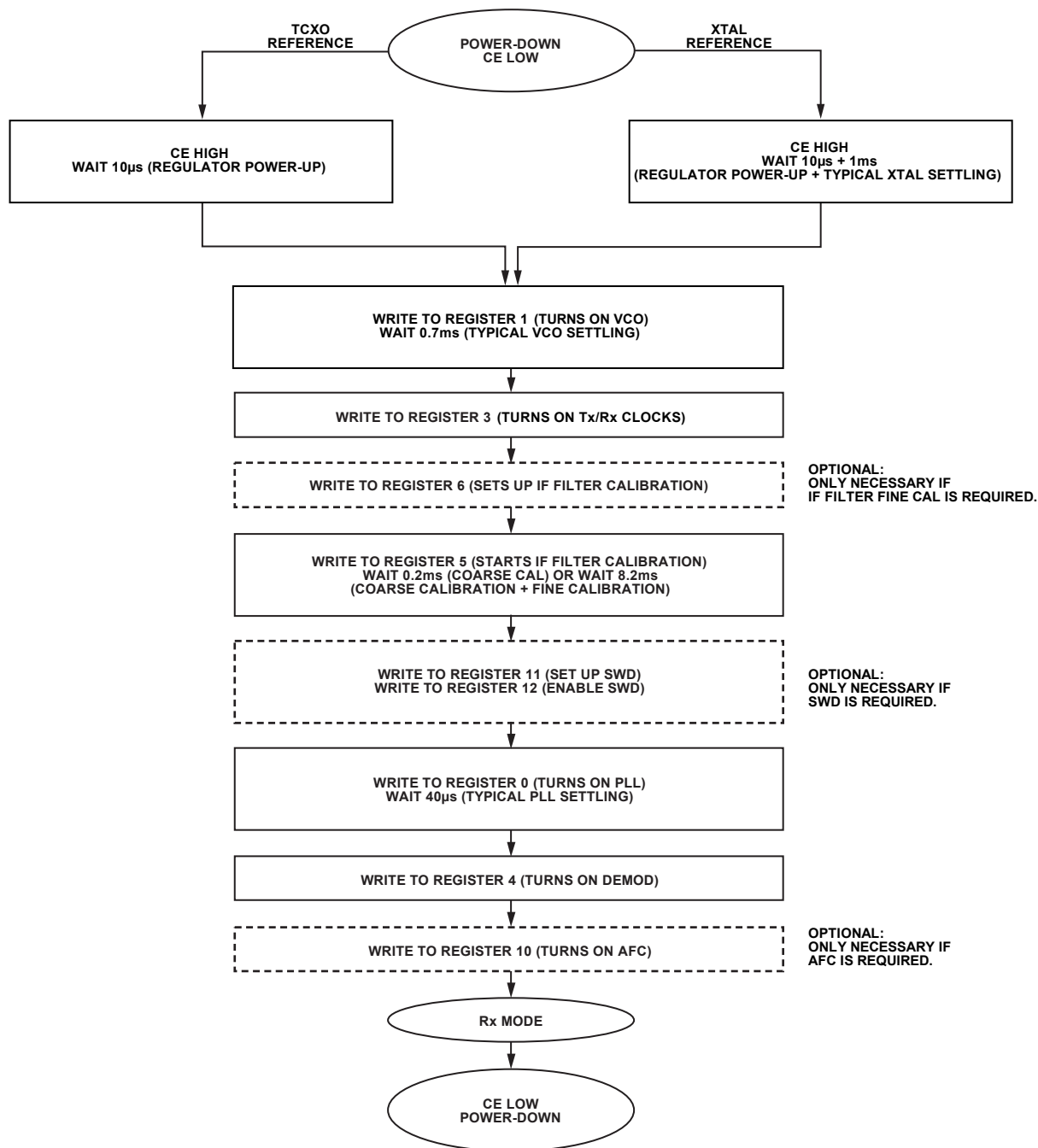
Figure 56. Power-Up Sequence for Receive Mode
