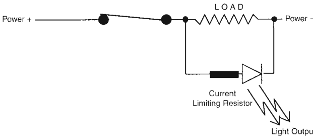
Figure 19. Wiring Diagram 4
