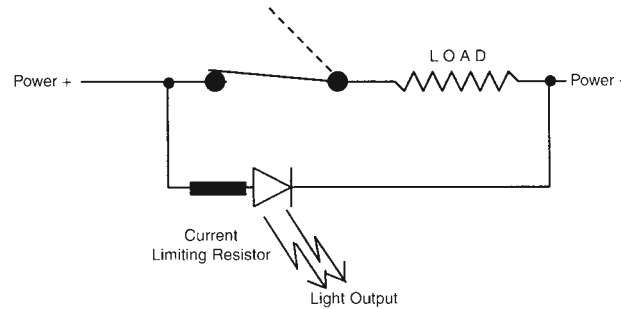
Figure 18. Wiring Diagram 3
