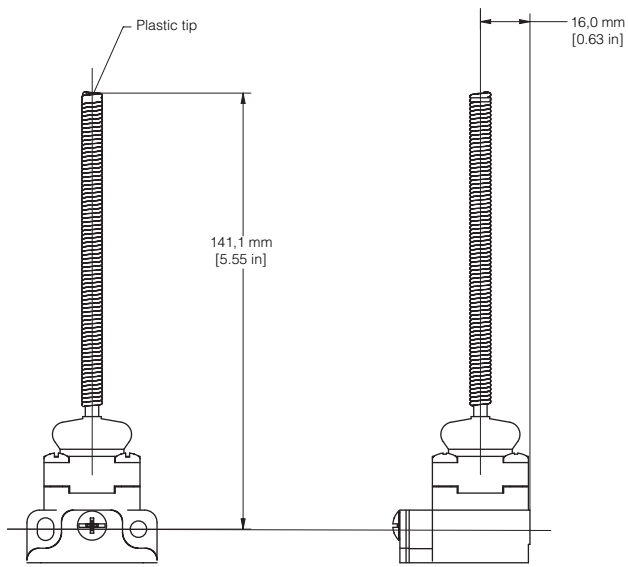
Figure 9. Coil Actuator
