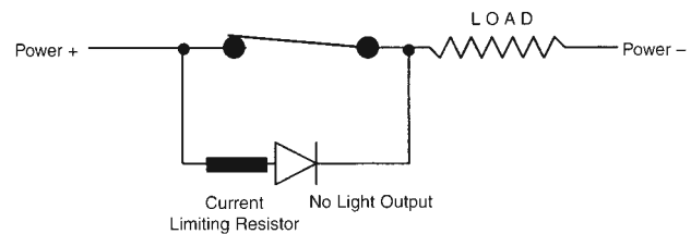
Figure 17. Wiring Diagram 2
