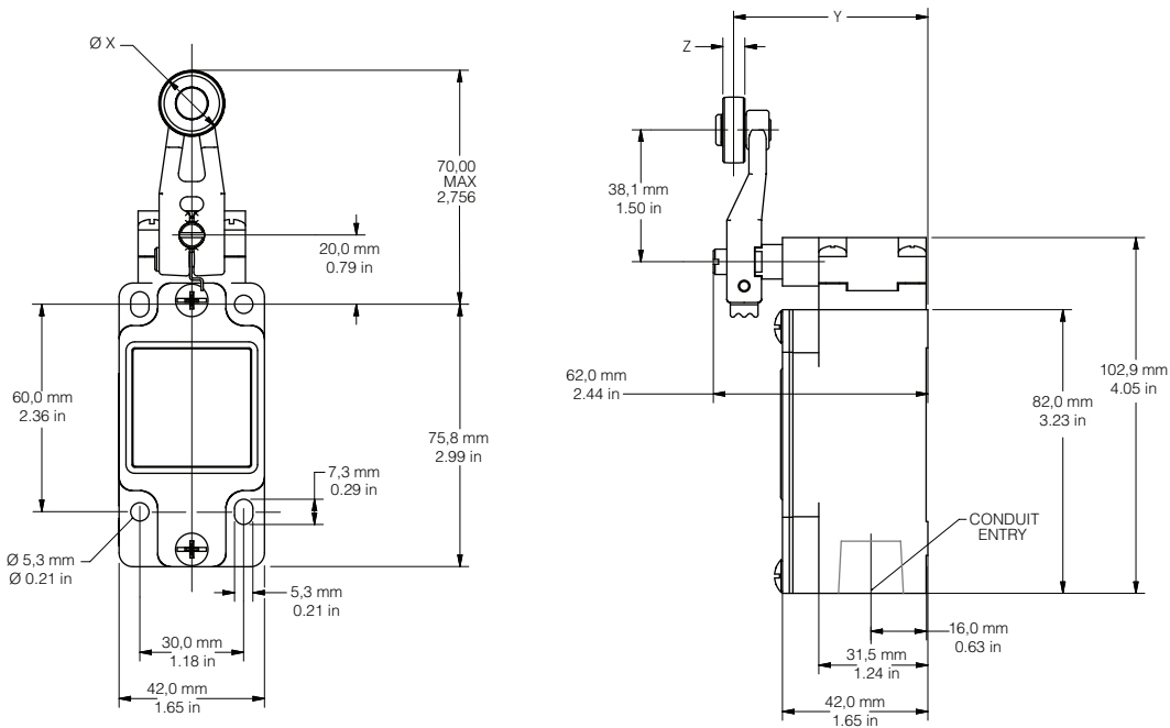
Figure 2. Fixed Lever, Side Rotary Switch - Non-plug-in Body Style, GLZ51 Style Lever, and GLA Body
