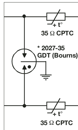
ITU-T K20 (Enhanced) Overcurrent Protection 4
