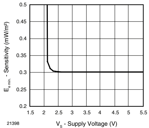
21398 Fig. 14 - Sensitivity vs. Supply Voltage
