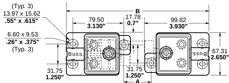
Dimensional Data \frac{\text{mm} (\pm .25)}{\text{Inches} (\pm .01)}
