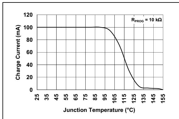
FIGURE 2-7: Charge Current ( I_{OUT} ) vs. Junction Temperature ( T_J ).
