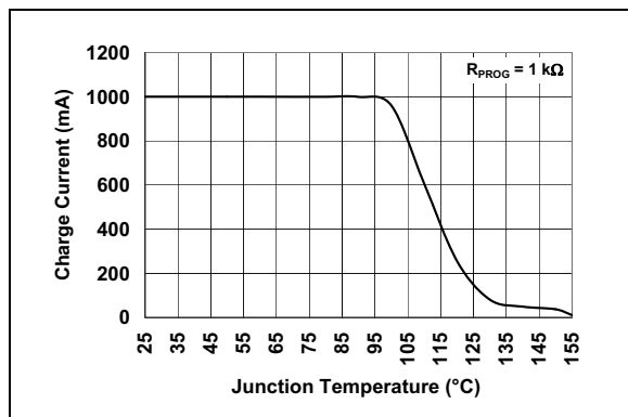
FIGURE 2-8: Charge Current ( I_{OUT} ) vs. Junction Temperature ( T_J ).
