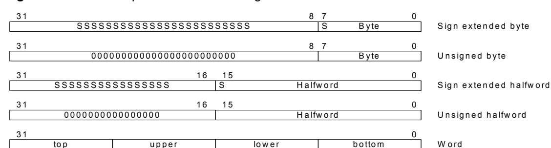
Figure 2-1. Data representation in the register file
