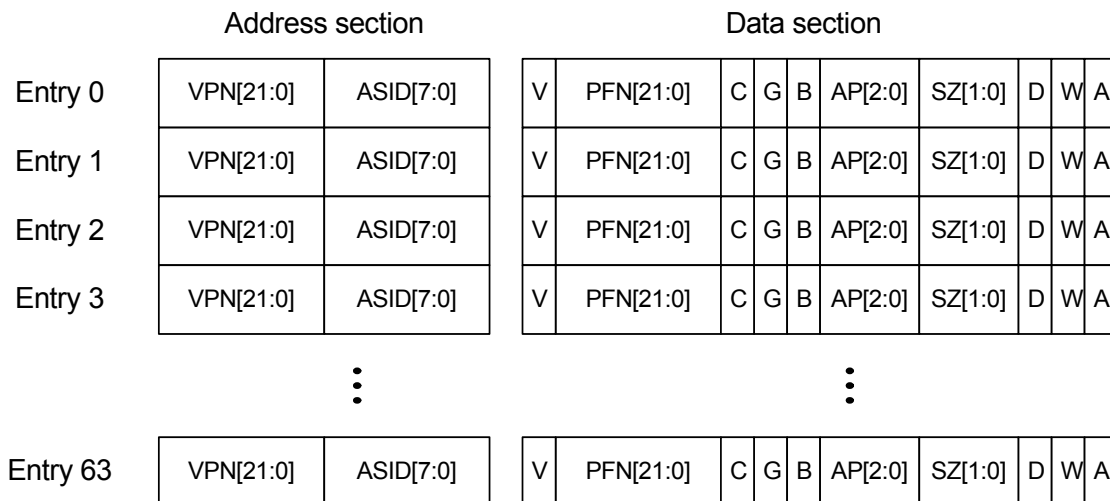
Figure 5-5. TLB organization
