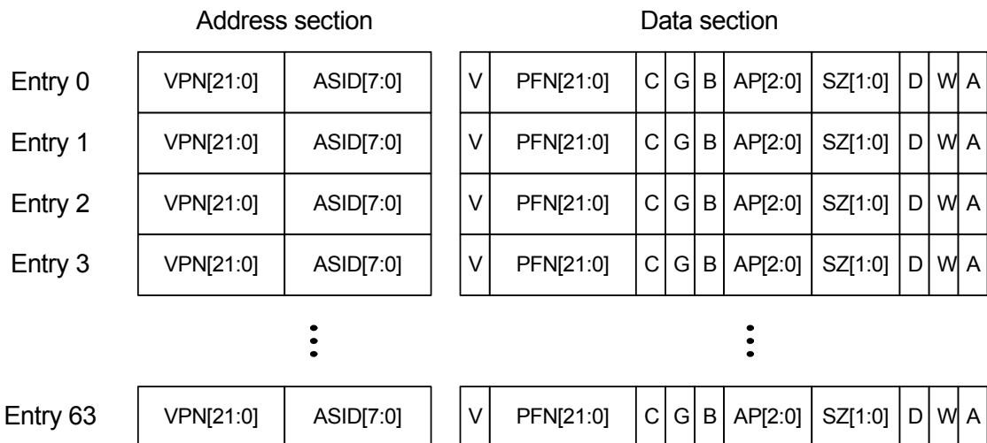
Figure 5-5. TLB organization
