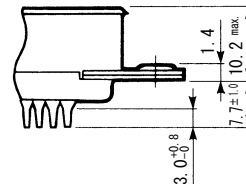
Dip solder
