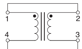
Parallel Hookup
