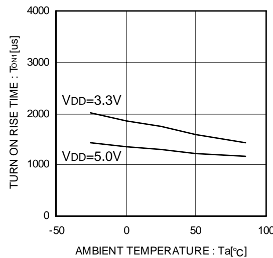
Figure 34. Output rise time
