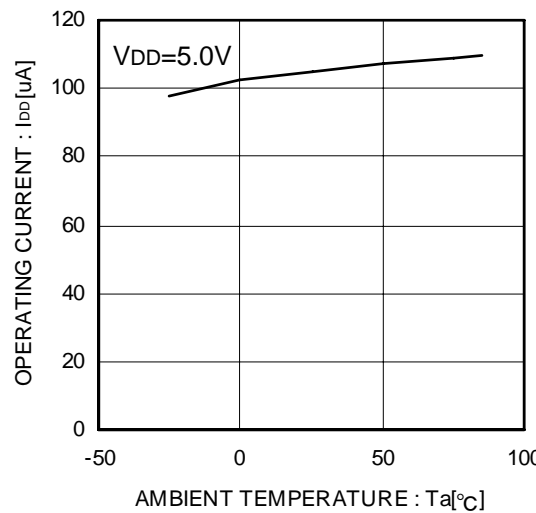
Figure 26. Operating current
