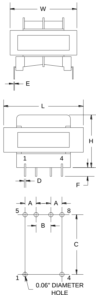
Board Layout
