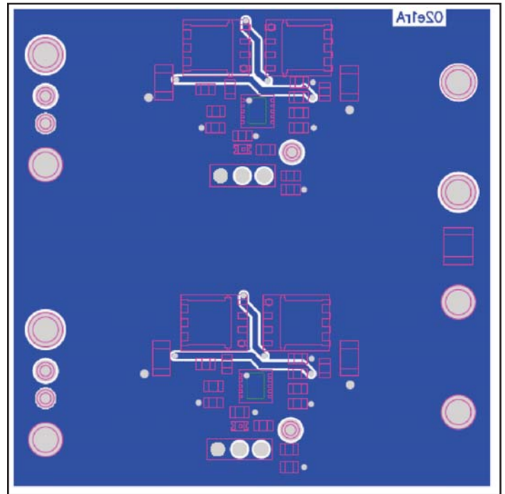
Figure 8b – PI2002-EVAL1 layout mid layer 2. Scale 2.0:1
