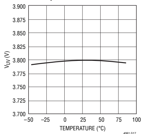
Undervoltage Lockout Voltage vs Temperature
