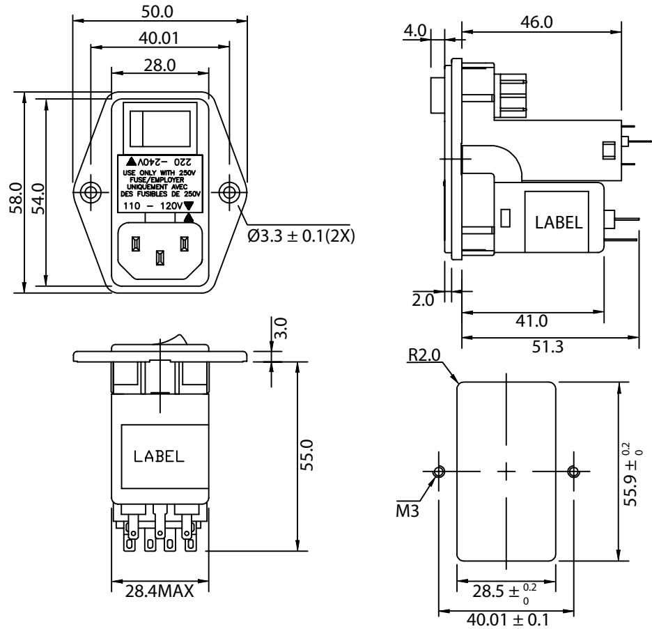
PANEL CUTOUT (MOUNTING FROM FRONT)
