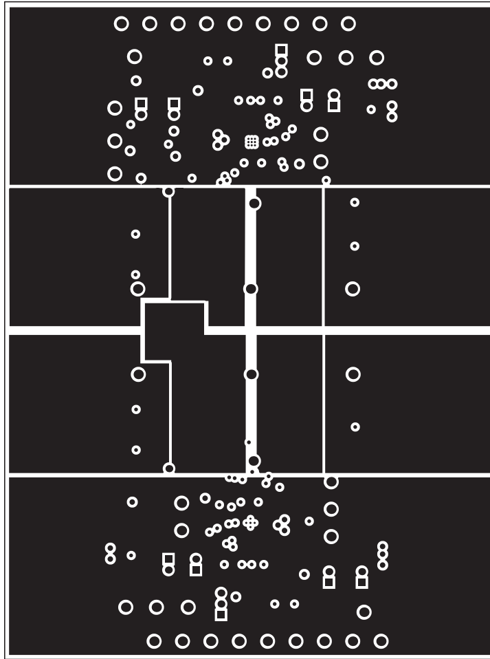
Figure 25. Midlayer 2 Routing
