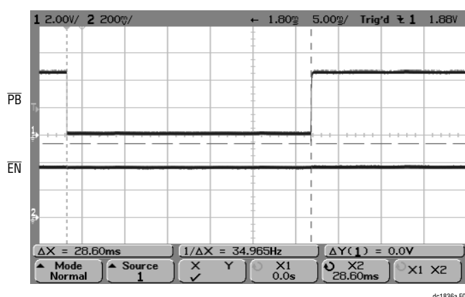
Figure 3. \overline{\text{PB}} Going Low for 28.6ms, and \overline{\text{EN}} Remaining High, Showing Too Short of a \overline{\text{PB}} Pulse to Properly Activate the Enable Pin
