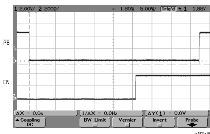
Figure 2. \overline{\text{PB}} Going Low For 46.1ms, and EN Pulling High, Showing a Proper Turn-On Sequence
