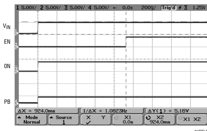
Figure 4. A Turn-On Sequence Where V_{\text{IN}} and ON Activate EN, as Opposed to PB. Notice the 924ms Delay Between V_{\text{IN}} Going High and EN Activating
