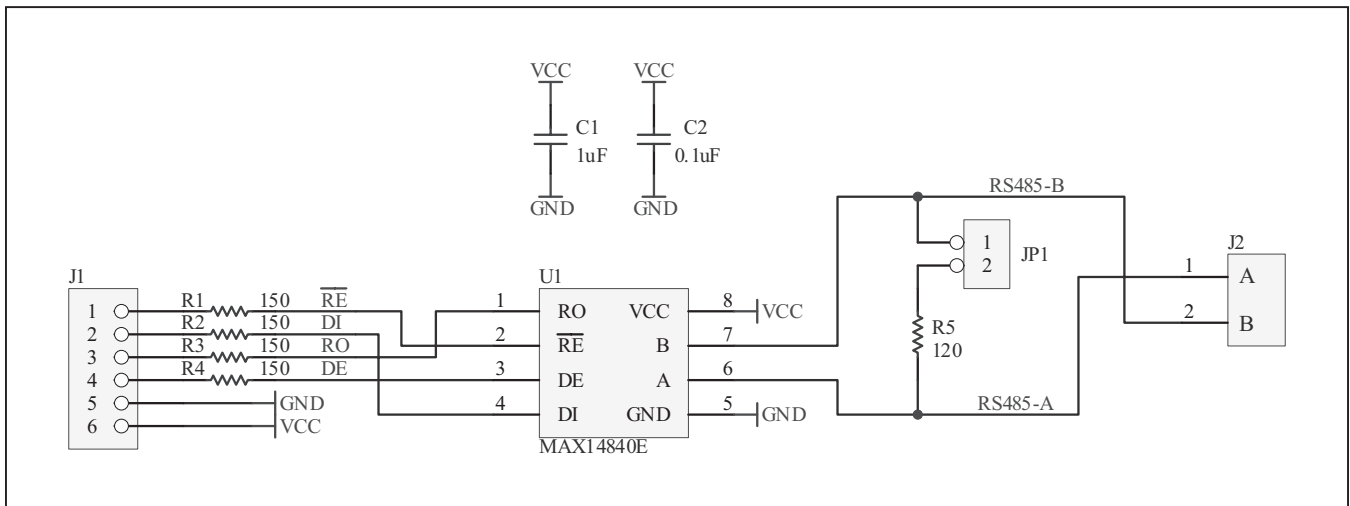
Figure 1. MAX14840PMB1 Peripheral Module Schematic
