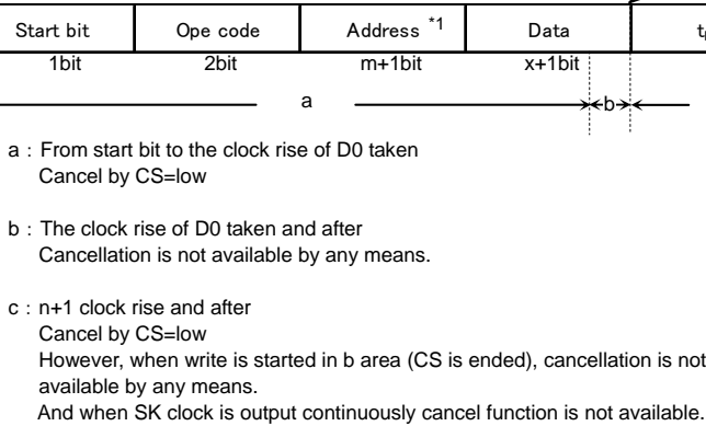
Figure 42. WRITE, WRAL cancel available timing
