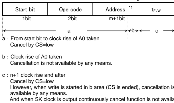
Figure 43. ERASE, ERAL cancel available timing
