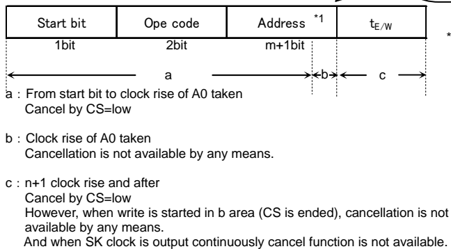
Figure 43. ERASE, ERAL cancel available timing
