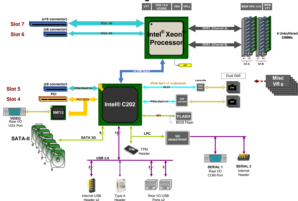
Figure 12. Intel® Server Board S1200BTS Functional Block Diagram
