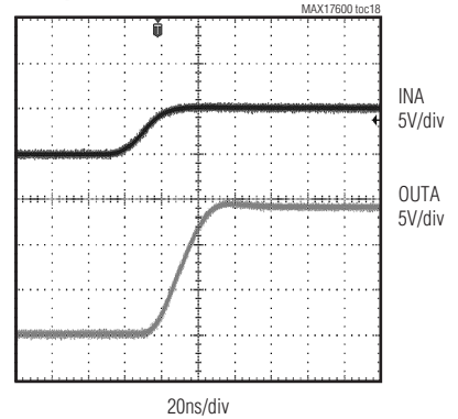
LOGIC INPUT VOLTAGE vs. OUTPUT VOLTAGE (MAX17604) ( V_{DD} = +14\text{V} , C_{OUTA} = 4.7\text{nF} )
