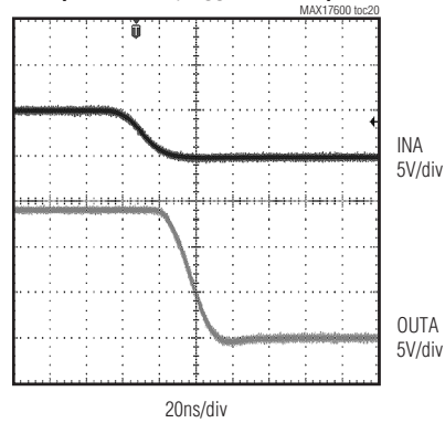
LOGIC INPUT VOLTAGE vs. OUTPUT VOLTAGE (MAX17604) ( V_{DD} = +14\text{V} , C_{OUTA} = 4.7\text{nF} )
