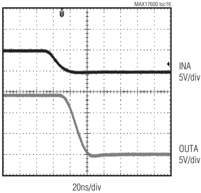
LOGIC INPUT VOLTAGE vs. OUTPUT VOLTAGE (MAX17604) ( V_{DD} = +14\text{V} , C_{OUTA} = 10\text{nF} )
