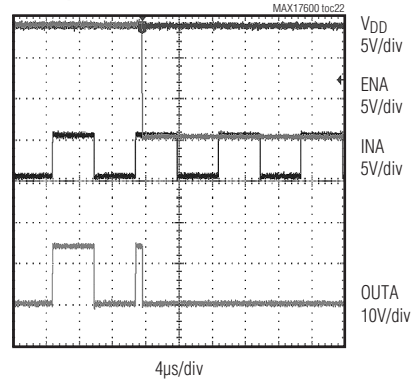
LOGIC OUTPUT vs. ENABLE ( V_{DD} = +14\text{V} , C_{OUTA} = 0\text{nF} )
