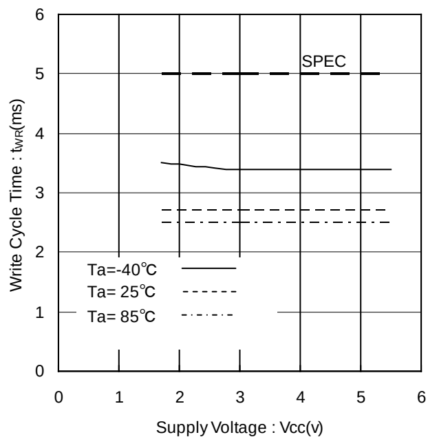
Figure 29. Write Cycle Time vs Supply Voltage
