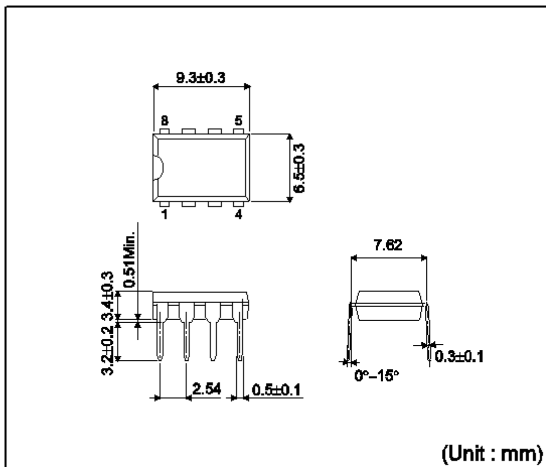
DIP-T8
