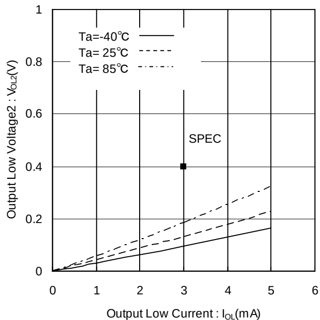
Figure 7. Output Low Voltage2 vs Output Low Current (V&lt;sub&gt;CC&lt;/sub&gt;=1.7V)
