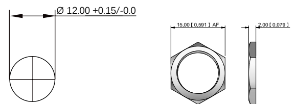
PANEL CUTOUT
