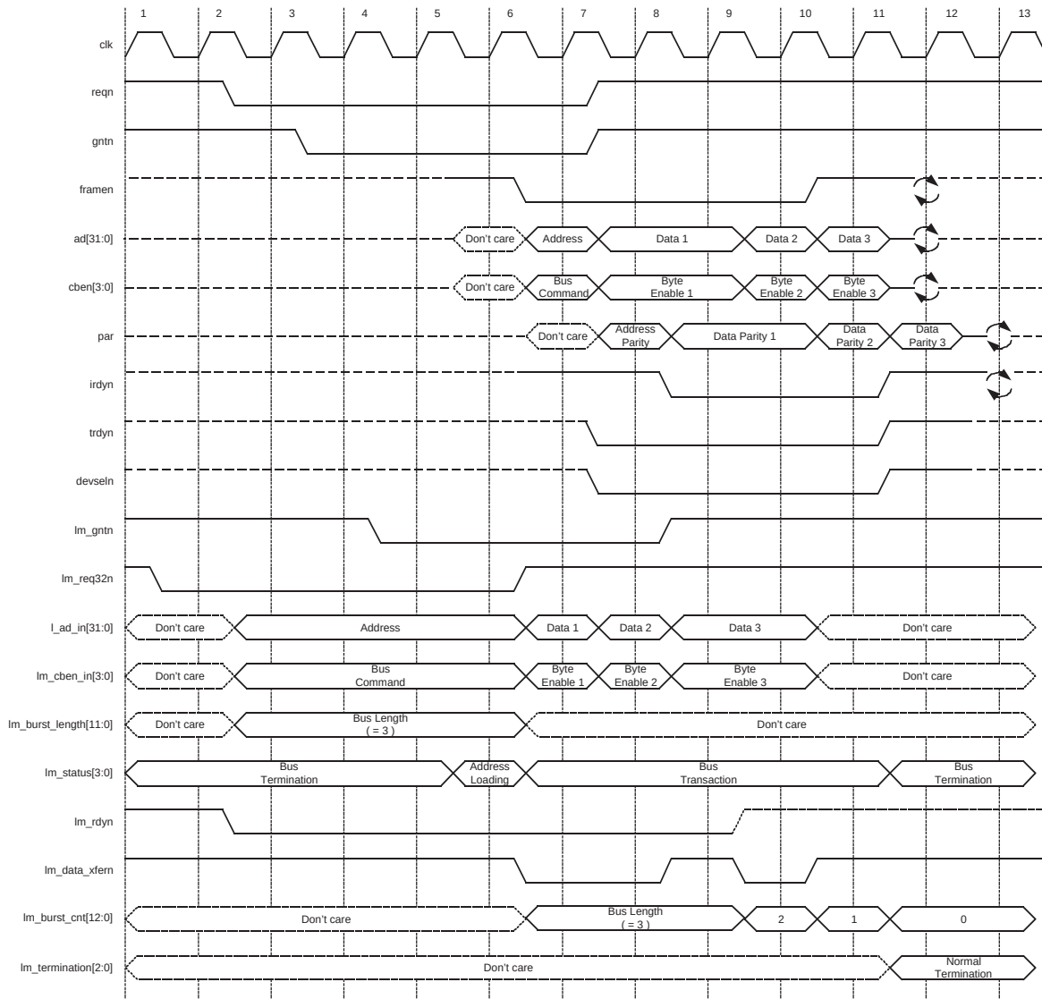
Figure 2-16. 32-bit Master Burst Write Transaction with a 32-bit Local Interface
