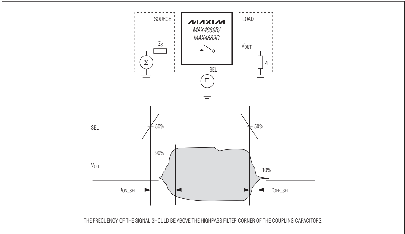
Figure 1. Switching Time
