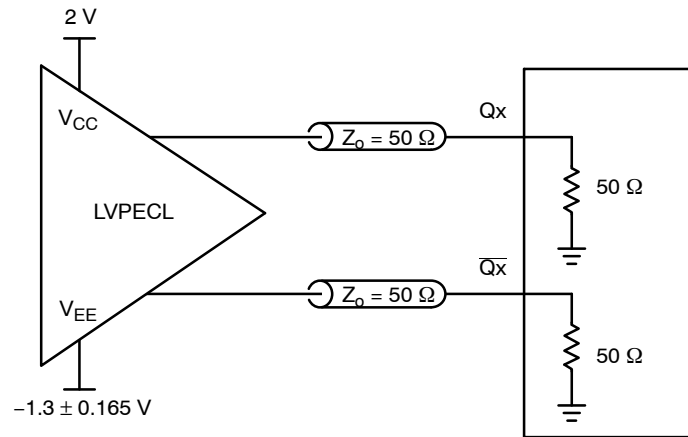
Figure 4. Typical Test Setup and Termination for Evaluation. A split supply of V_{CC} = 2.0 \text{ V} and V_{EE} = -1.3 \pm 0.165 \text{ V} allows a convenient direct connection termination into typical oscilloscope 50 \Omega to GND impedance modules. For Application termination schemes see AND8020.
