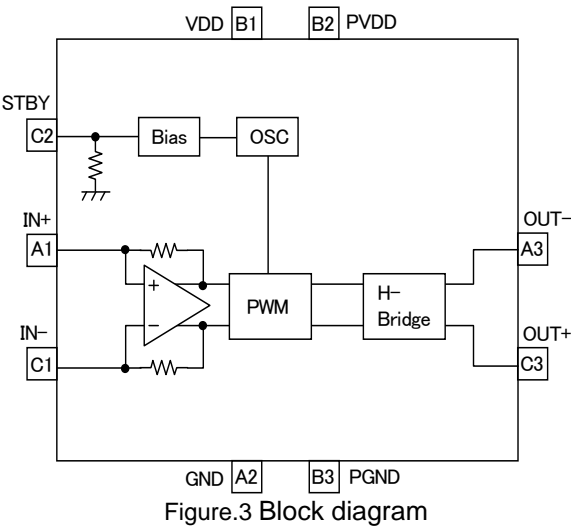
Figure.3 Block diagram
