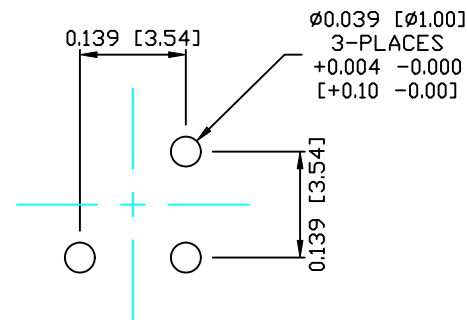
PLC LAYOUT
